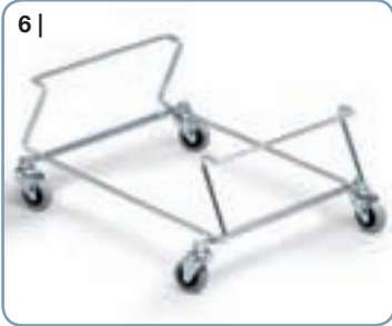
6 | TROLLEY SHOPPING BASKET 19 Galvanized carrier with reversible wheels. Dimensions: 420x340x200 mm (LxWxH) # 1801565000 silver 📦 1 piece
